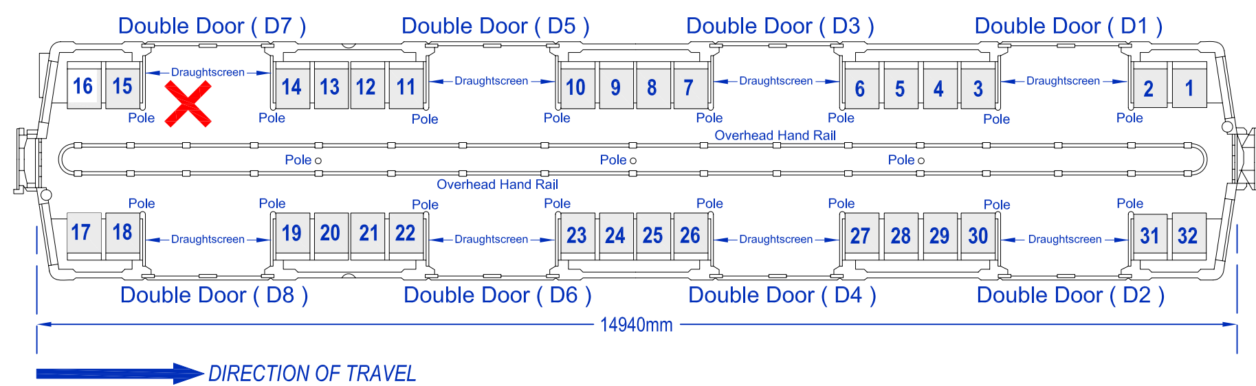
Second Carriage ( Trailer Car ) - Plan View
