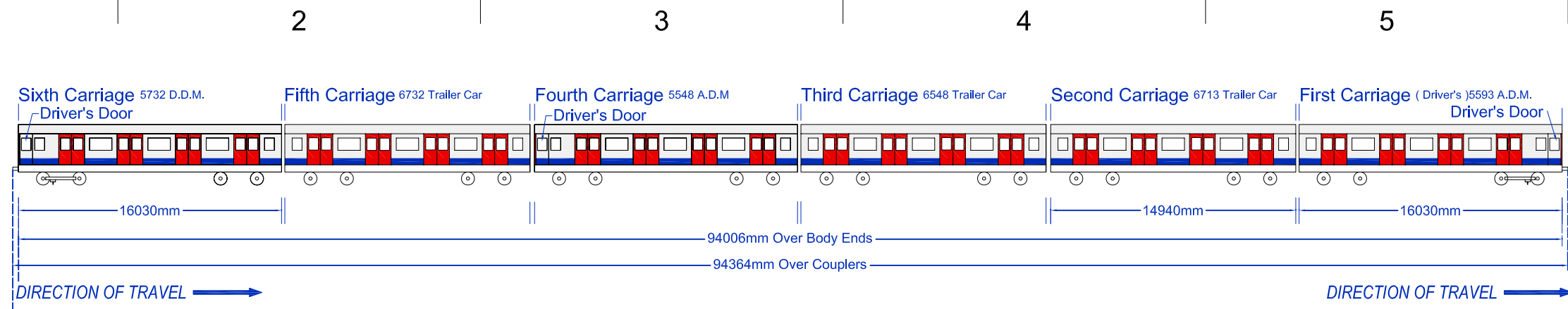
Six Car Train C69 / 77 Surface Stock - Circle Line - Side Elevation
