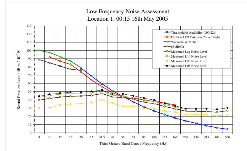
LFN Audibility External Facade 16/05/05 Figure 4
