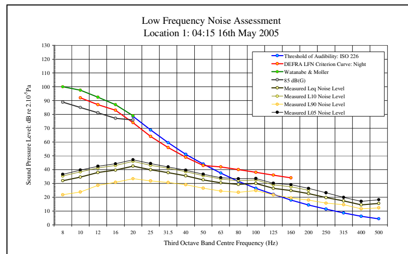
LFN Audibility External Facade 16/05/05 Figure 52
