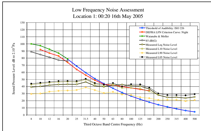
LFN Audibility External Facade 16/05/05 Figure 5
