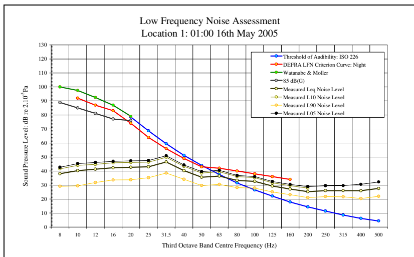
LFN Audibility External Facade 16/05/05 Figure 13
