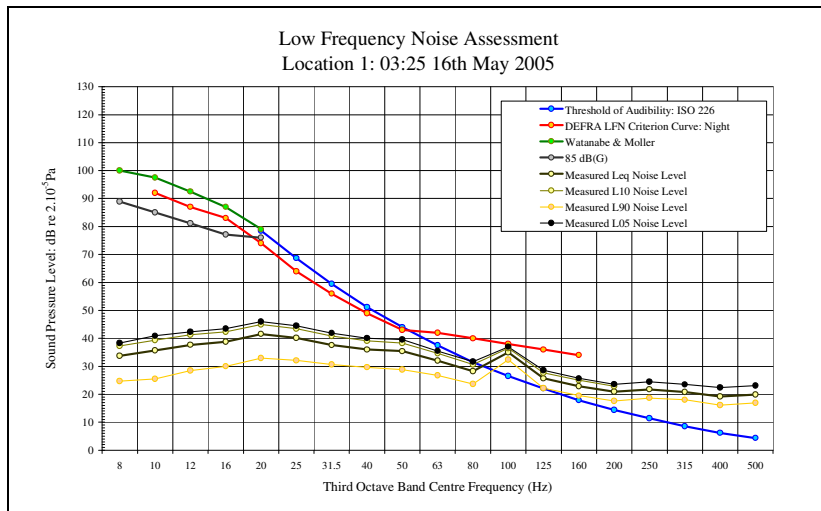
LFN Audibility External Facade 16/05/05 Figure 42
