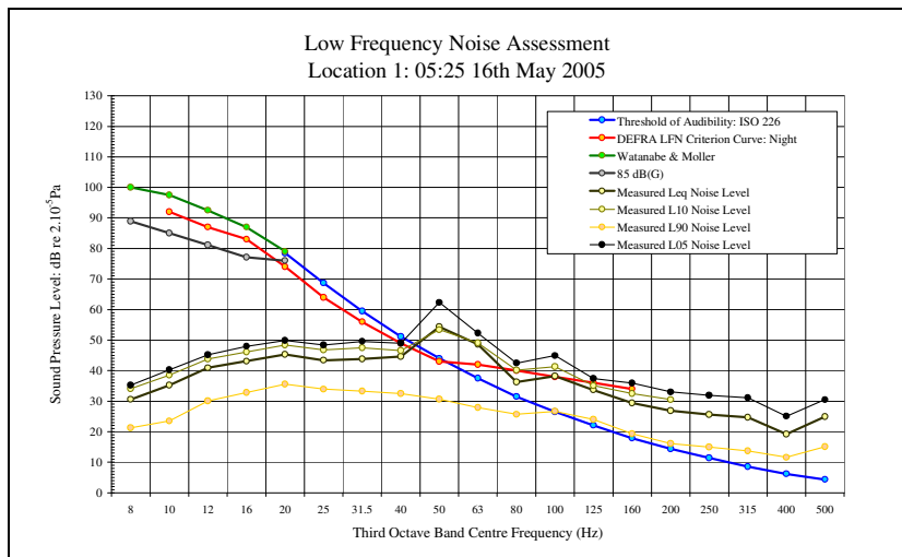
LFN Audibility External Facade 16/05/05 Figure 66
