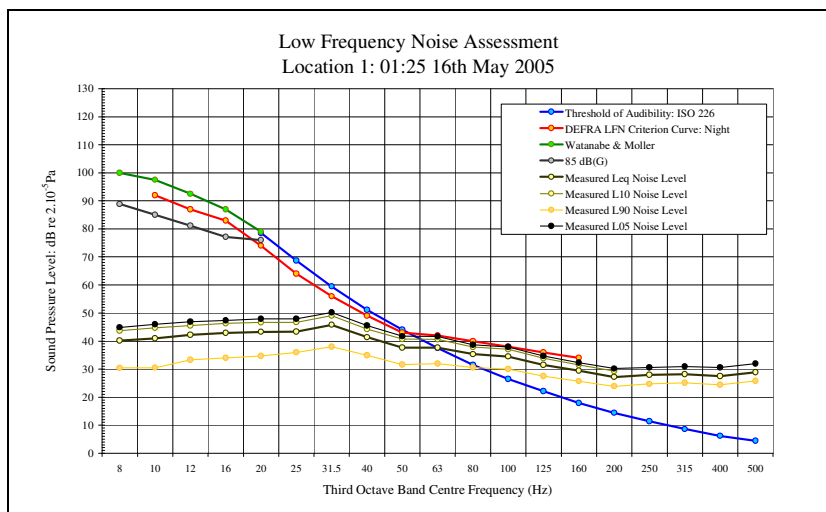
LFN Audibility External Facade 16/05/05 Figure 18
