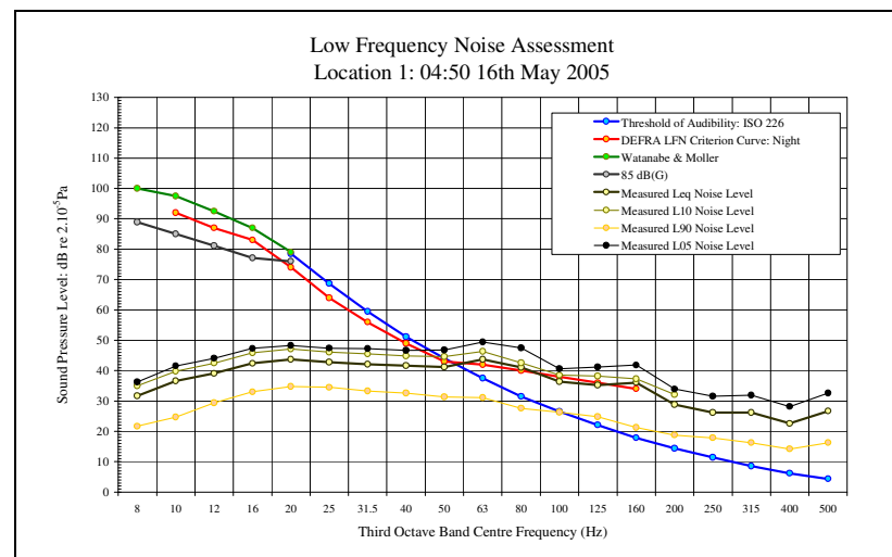
LFN Audibility External Facade 16/05/05 Figure 59
