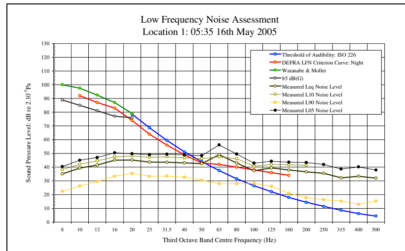
LFN Audibility External Facade 16/05/05 Figure 68
