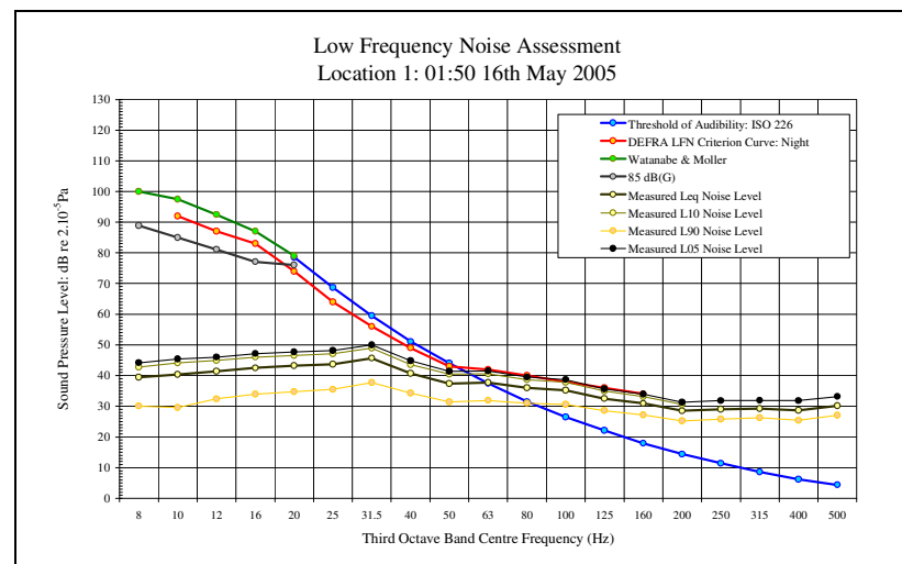
LFN Audibility External Facade 16/05/05 Figure 23
