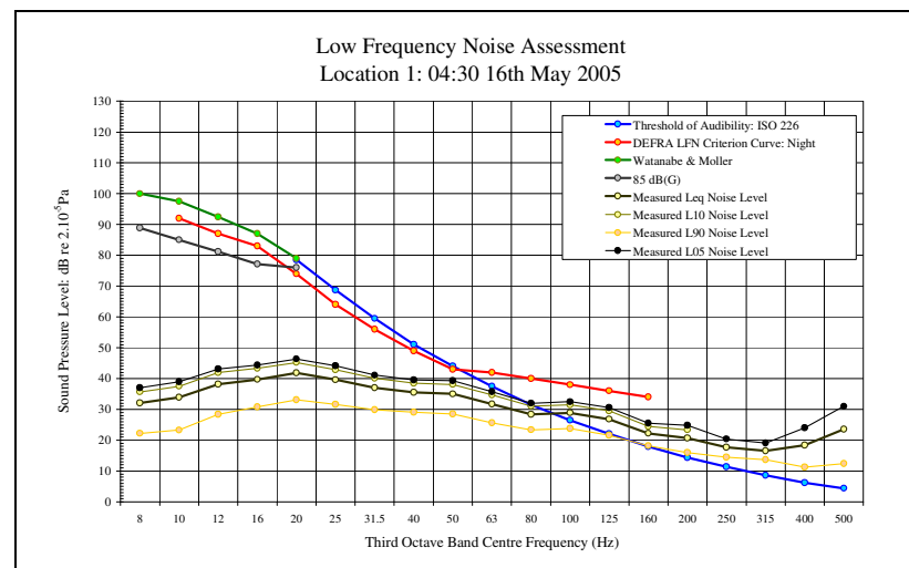
LFN Audibility External Facade 16/05/05 Figure 55
