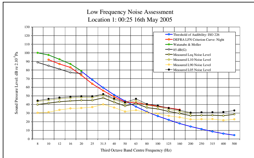
LFN Audibility External Facade 16/05/05 Figure 6
