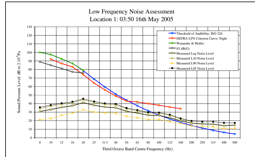
LFN Audibility External Facade 16/05/05 Figure 47
