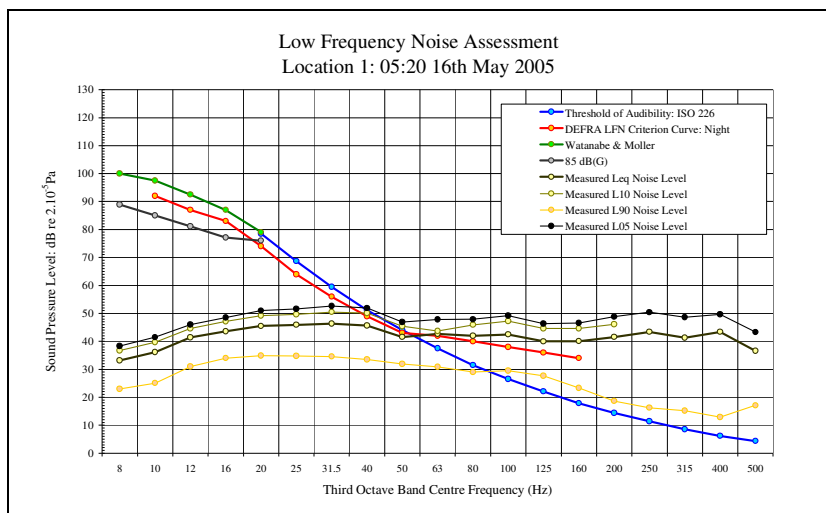
LFN Audibility External Facade 16/05/05 Figure 65
