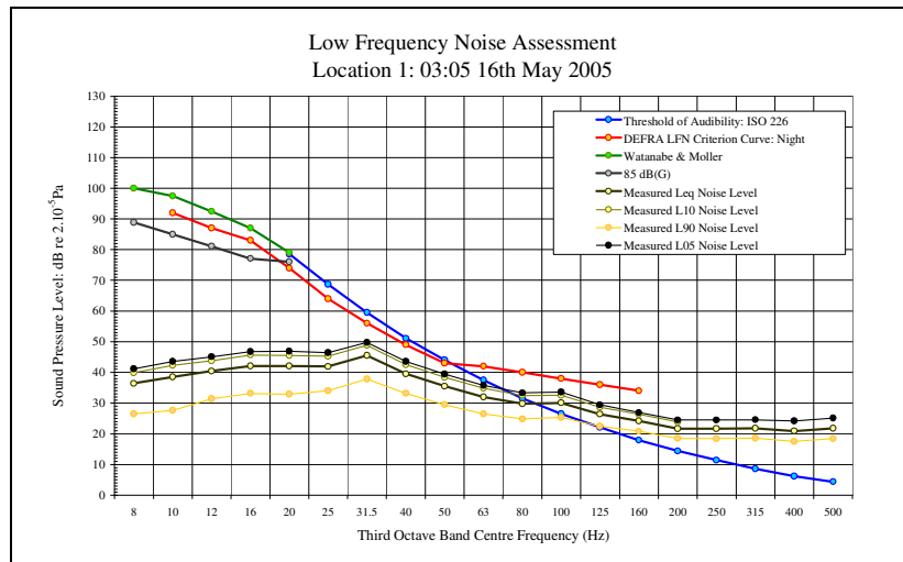
LFN Audibility External Facade 16/05/05 Figure 38
