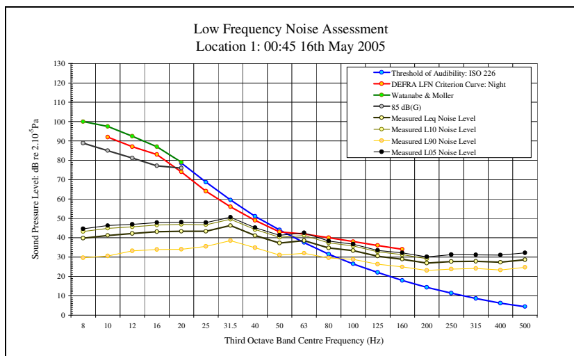
LFN Audibility External Facade 16/05/05 Figure 10
