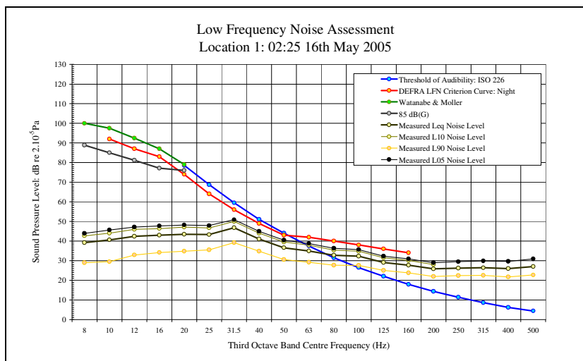
LFN Audibility External Facade 16/05/05 Figure 30
