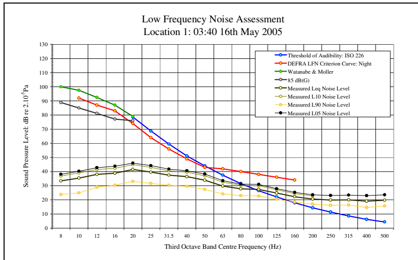
LFN Audibility External Facade 16/05/05 Figure 45
