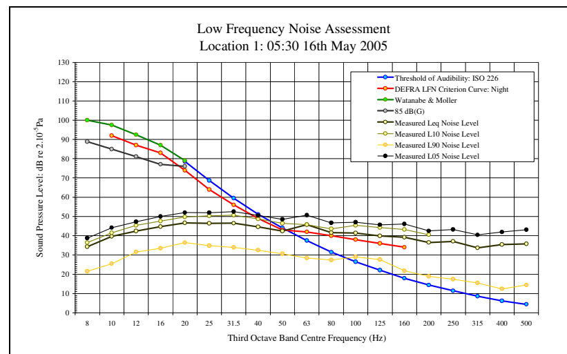
LFN Audibility External Facade 16/05/05 Figure 67
