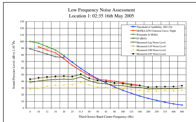
LFN Audibility External Facade 16/05/05 Figure 32
