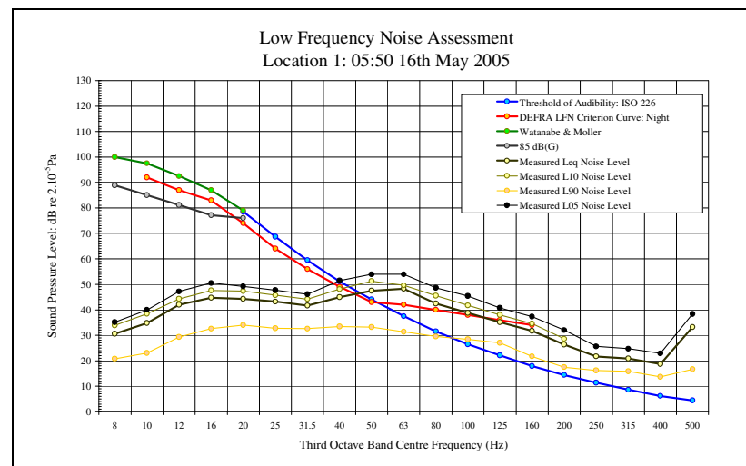
LFN Audibility External Facade 16/05/05 Figure 71
