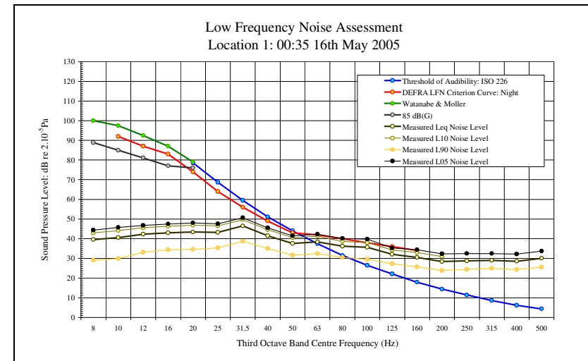
LFN Audibility External Facade 16/05/05 Figure 8
