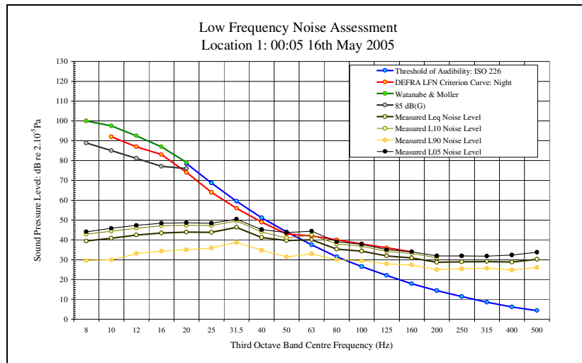
LFN Audibility External Facade 16/05/05 Figure 2
