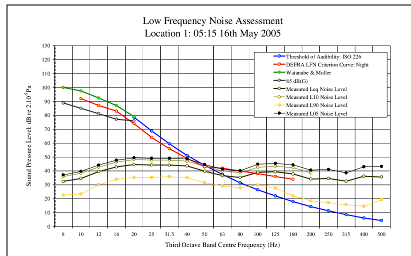
LFN Audibility External Facade 16/05/05 Figure 64
