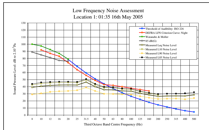
LFN Audibility External Facade 16/05/05 Figure 20
