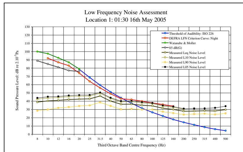
LFN Audibility External Facade 16/05/05 Figure 19
