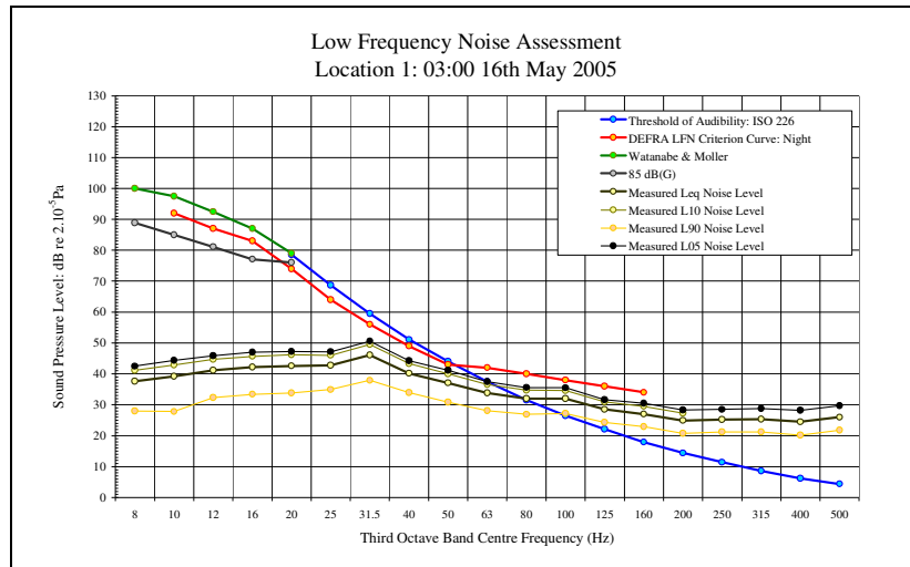
LFN Audibility External Facade 16/05/05 Figure 37
