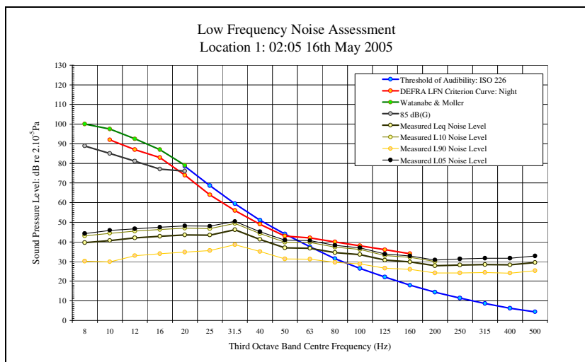
LFN Audibility External Facade 16/05/05 Figure 26
