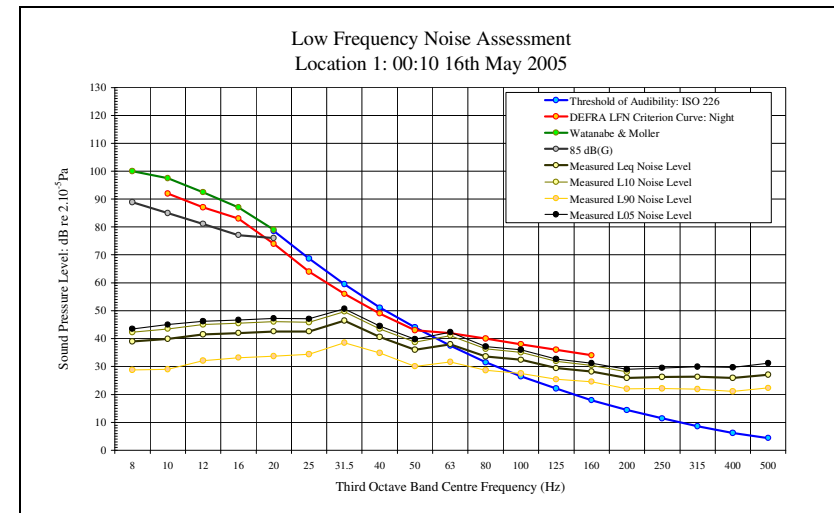
LFN Audibility External Facade 16/05/05 Figure 3
