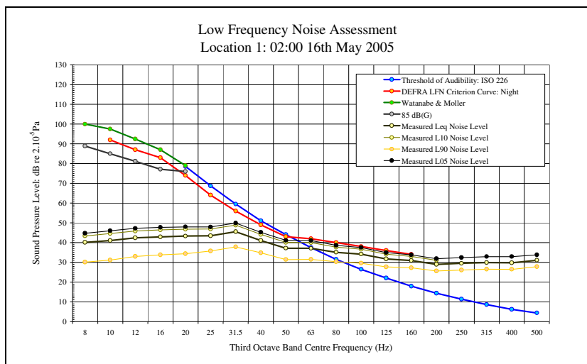
LFN Audibility External Facade 16/05/05 Figure 25
