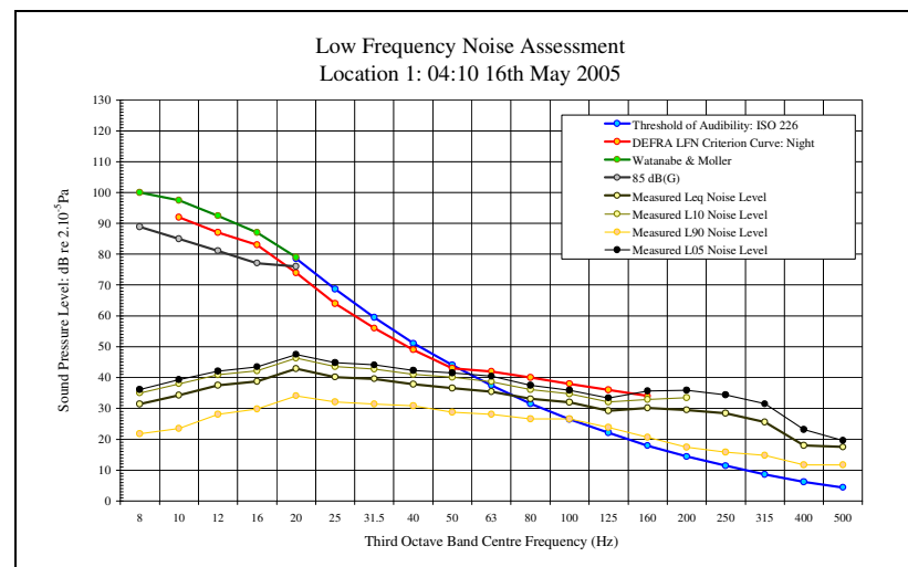
LFN Audibility External Facade 16/05/05 Figure 51
