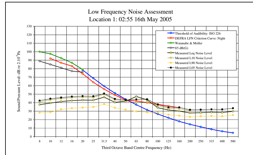
LFN Audibility External Facade 16/05/05 Figure 36
