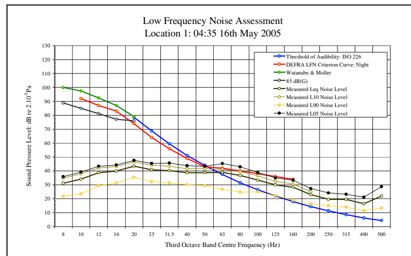
LFN Audibility External Facade 16/05/05 Figure 56
