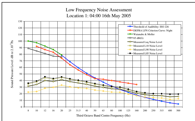
LFN Audibility External Facade 16/05/05 Figure 49
