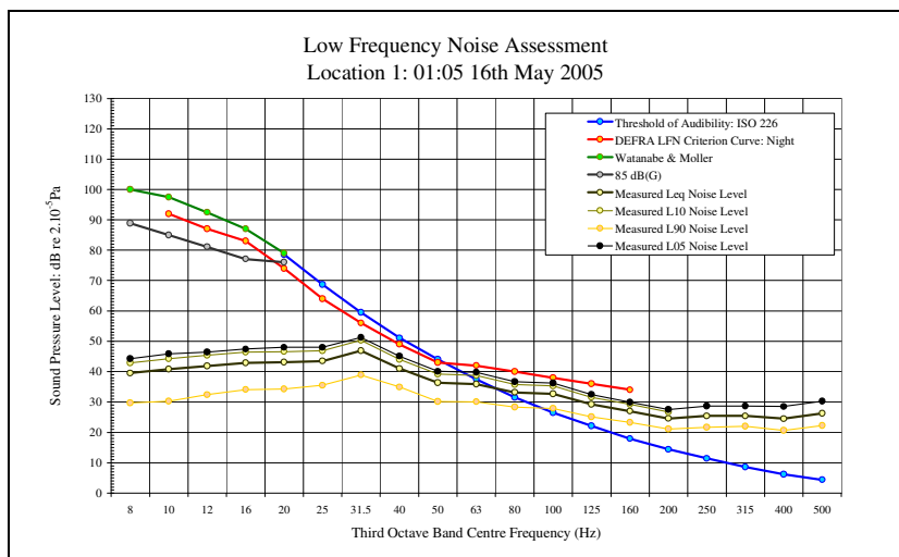
LFN Audibility External Facade 16/05/05 Figure 14
