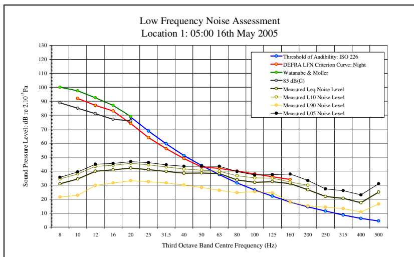
LFN Audibility External Facade 16/05/05 Figure 61
