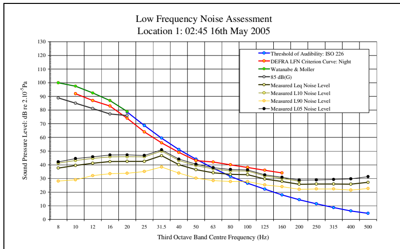
LFN Audibility External Facade 16/05/05 Figure 34
