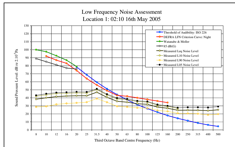
LFN Audibility External Facade 16/05/05 Figure 27
