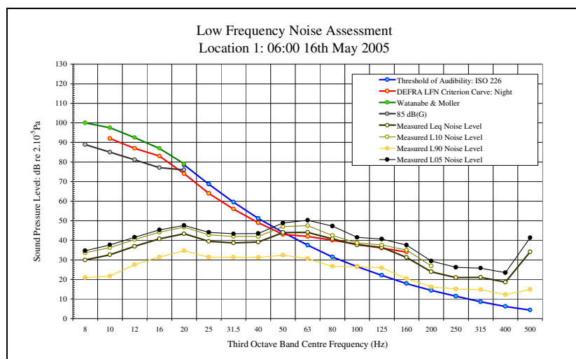
LFN Audibility External Facade 16/05/05 Figure 73
