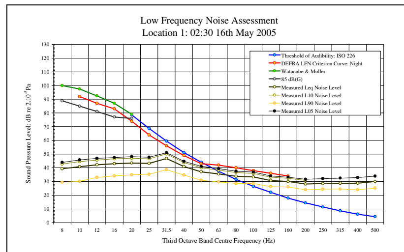
LFN Audibility External Facade 16/05/05 Figure 31
