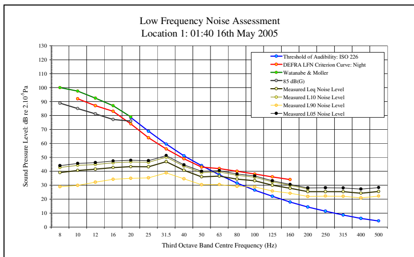
LFN Audibility External Facade 16/05/05 Figure 21
