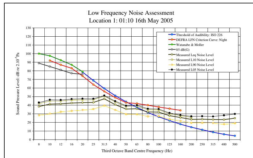
LFN Audibility External Facade 16/05/05 Figure 15
