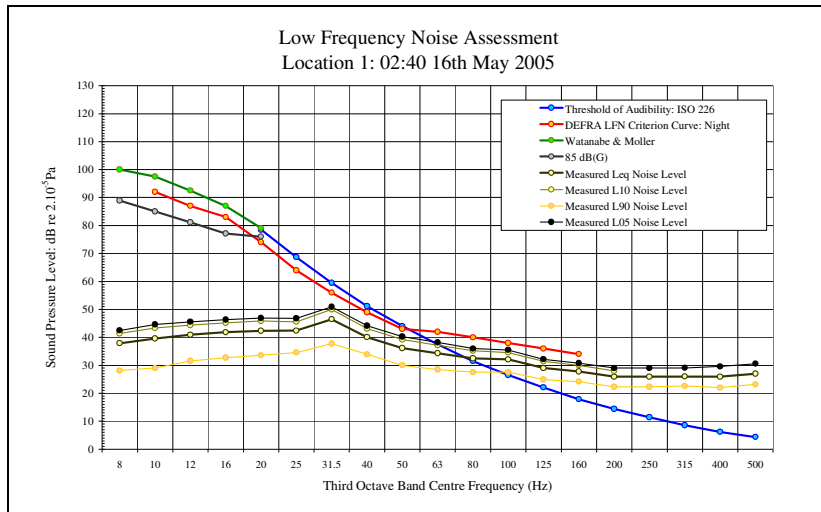
LFN Audibility External Facade 16/05/05 Figure 33
