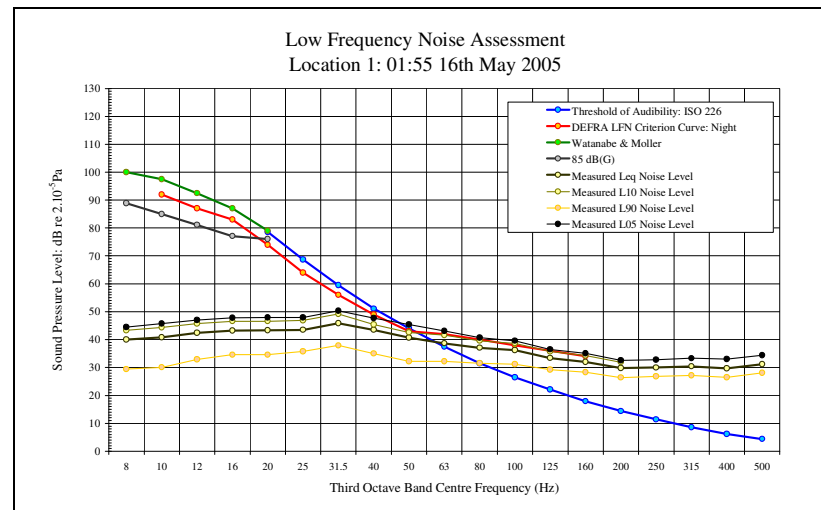
LFN Audibility External Facade 16/05/05 Figure 24
