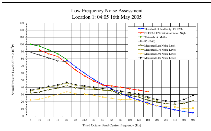
LFN Audibility External Facade 16/05/05 Figure 50
