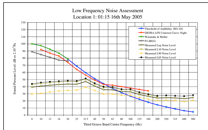
LFN Audibility External Facade 16/05/05 Figure 16
