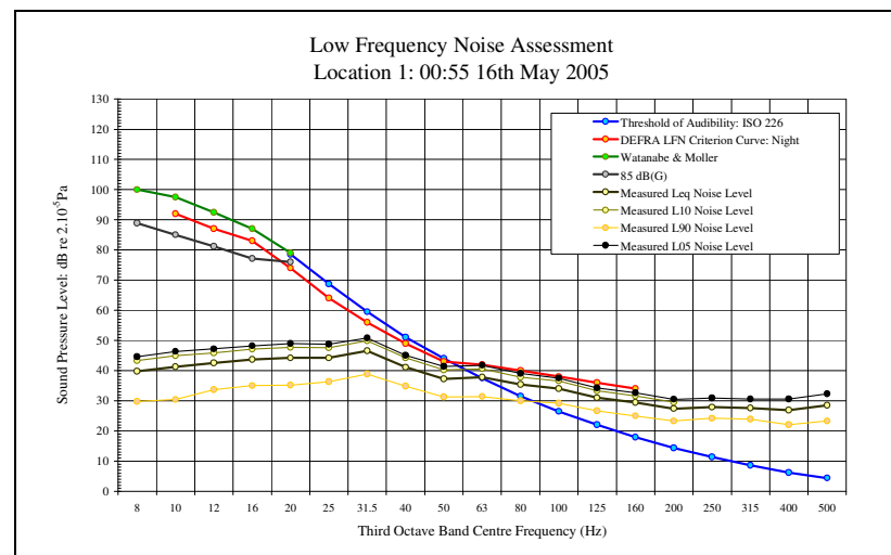
LFN Audibility External Facade 16/05/05 Figure 12
