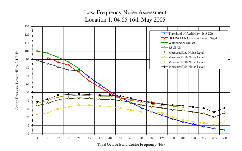
LFN Audibility External Facade 16/05/05 Figure 60
