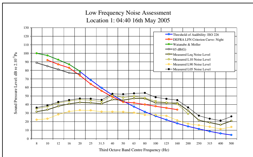
LFN Audibility External Facade 16/05/05 Figure 57
