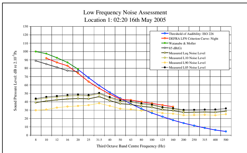
LFN Audibility External Facade 16/05/05 Figure 29
