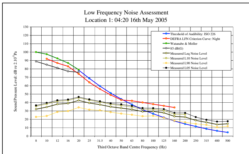
LFN Audibility External Facade 16/05/05 Figure 53
