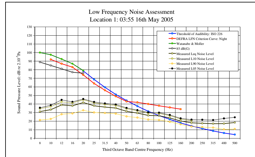
LFN Audibility External Facade 16/05/05 Figure 48
