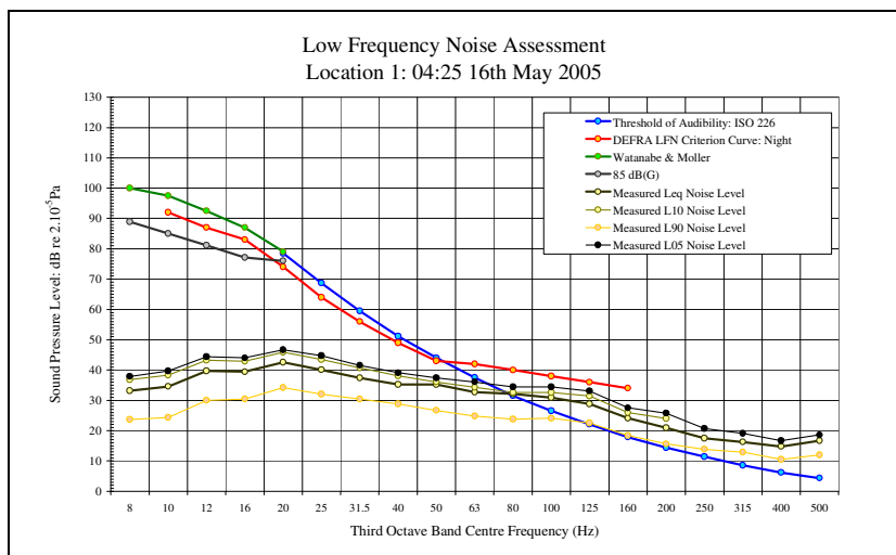
LFN Audibility External Facade 16/05/05 Figure 54
