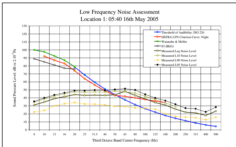
LFN Audibility External Facade 16/05/05 Figure 69
