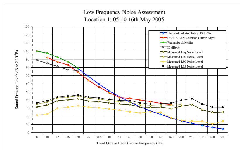
LFN Audibility External Facade 16/05/05 Figure 63
