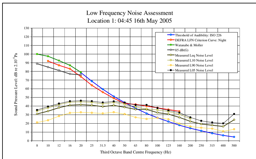
LFN Audibility External Facade 16/05/05 Figure 58
