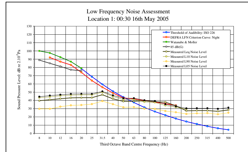
LFN Audibility External Facade 16/05/05 Figure 7
