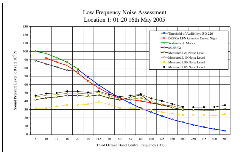
LFN Audibility External Facade 16/05/05 Figure 17
