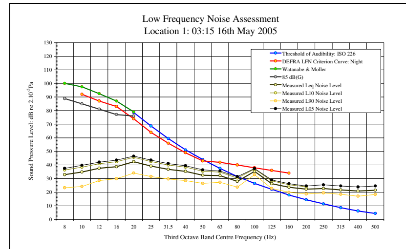
LFN Audibility External Facade 16/05/05 Figure 40
