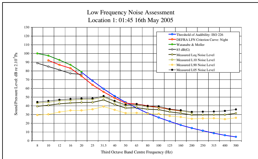
LFN Audibility External Facade 16/05/05 Figure 22
