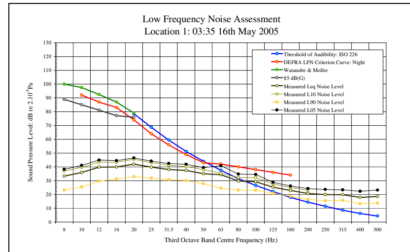
LFN Audibility External Facade 16/05/05 Figure 44
