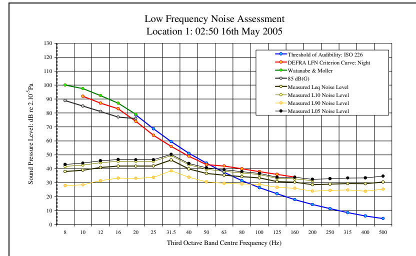
LFN Audibility External Facade 16/05/05 Figure 35
