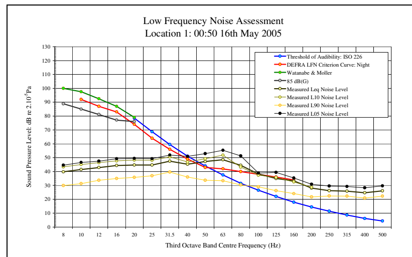
LFN Audibility External Facade 16/05/05 Figure 11
