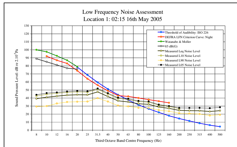
LFN Audibility External Facade 16/05/05 Figure 28
