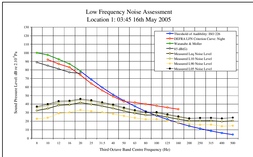
LFN Audibility External Facade 16/05/05 Figure 46
