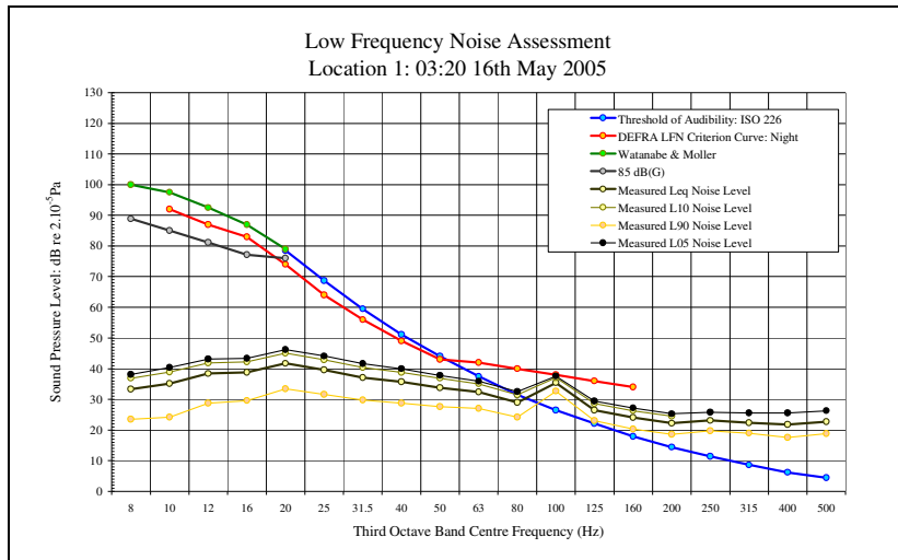
LFN Audibility External Facade 16/05/05 Figure 41
