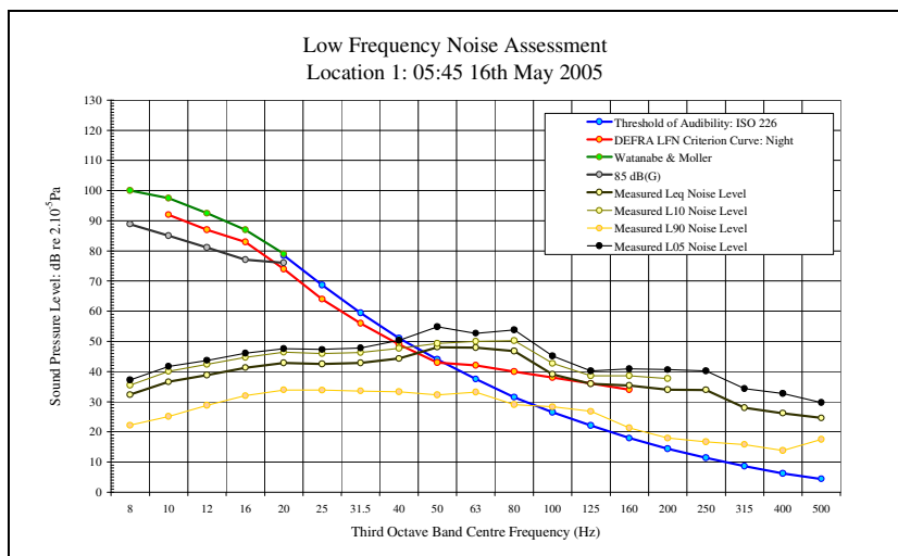
LFN Audibility External Facade 16/05/05 Figure 70
