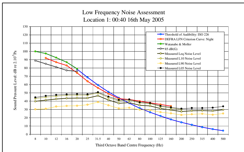
LFN Audibility External Facade 16/05/05 Figure 9
