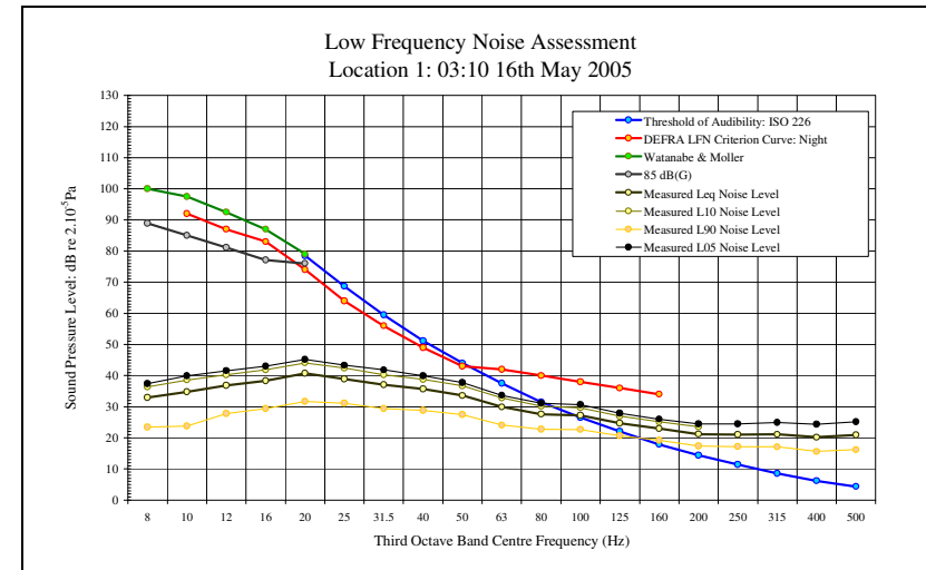
LFN Audibility External Facade 16/05/05 Figure 39
