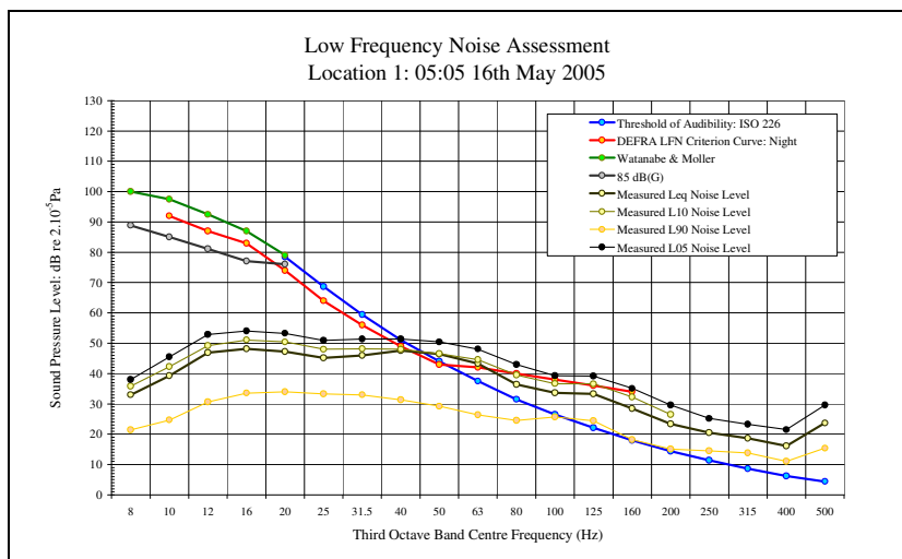
LFN Audibility External Facade 16/05/05 Figure 62
