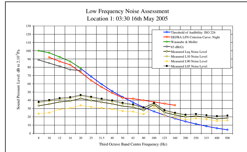
LFN Audibility External Facade 16/05/05 Figure 43
