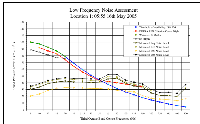
LFN Audibility External Facade 16/05/05 Figure 72
