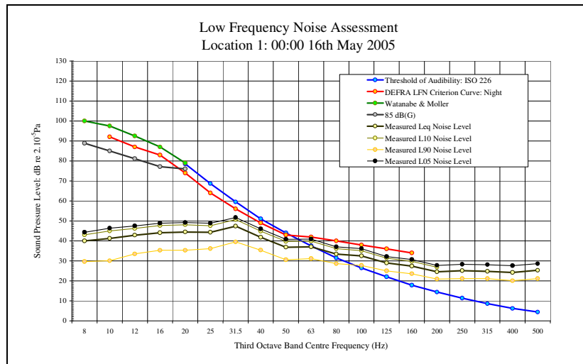
LFN Audibility External Facade 16/05/05 Figure 1
