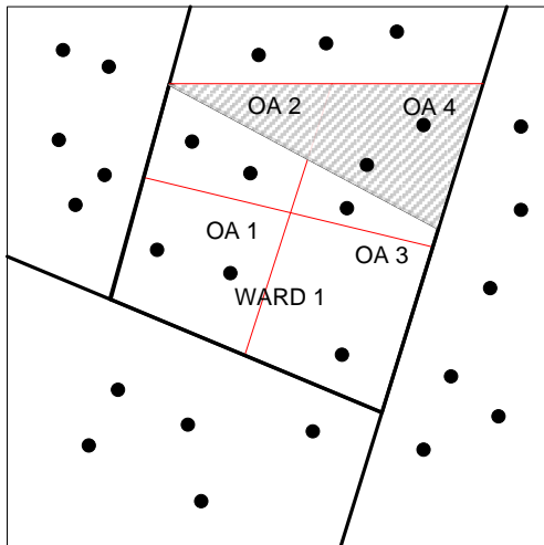
Fig 2. In 2011, the difference between WARD 1 and the OAs means a disclosive sliver is produced
