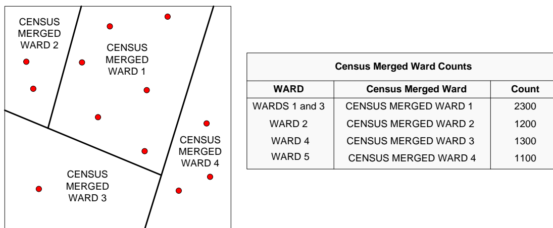
Fig 8. WARD 1 has been merged with WARD 3 to increase the population count to a non-disclosive level. This has been done as WARD 3 contains the nearest OA population weighted centroid to WARD 1
