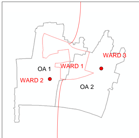
Fig 3. Best fit showing a ward (WARD 1) with a small population. As it contains no OA population weighted centroids, it would not be included in the best fit lookup without a manual adjustment being applied.
