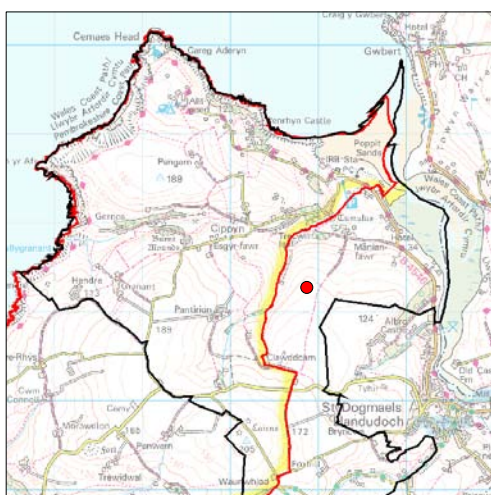
Fig 6. The villages within the national park boundary (red/yellow line) are excluded from any best fit counts for the national park as the population weighted centroid falls outside the park boundary
