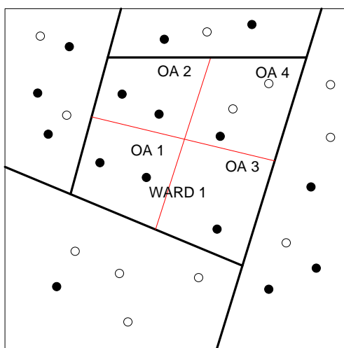
Fig 9. In 2011, households fit exactly into WARD 1. WARD 1 has 8 households
