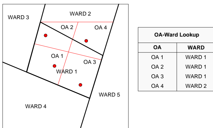
Fig 1. 2011 Best fit of Output Areas to Higher Geographies. OA4 is allocated to WARD 2 because OA4's population weighted centroid falls within the WARD 2 boundary
