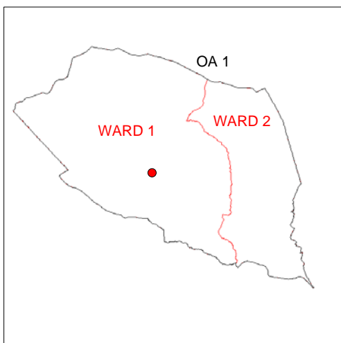
Fig 4. Best fit showing a ward (WARD 2) with a small population contained within a single OA. For 2011, as the ward is within a single OA, it will be allocated the OA centroid nearest to its boundary
