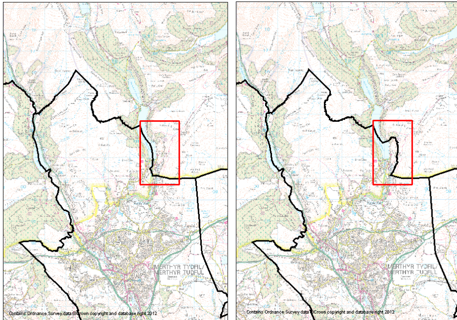
Fig 5. Changes in the local authority boundary for Merthyr Tydfil between 2003 and 2011
