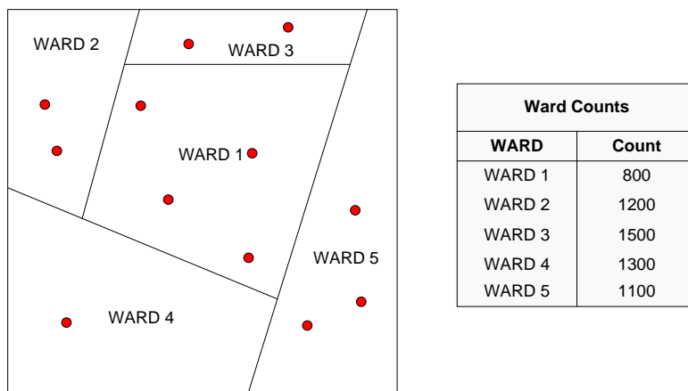
Fig 7. Ward estimates best fitted from the OA population weighted centroid. As WARD 1 contains less than 1000 population, it will need to be merged to provide enough population to take it above the lower threshold.
