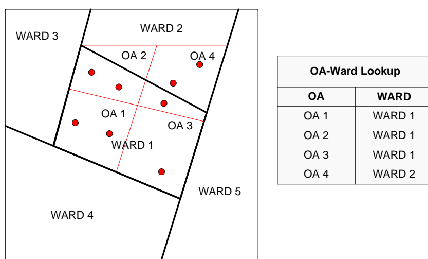
Fig 10. 2001 Best fit of Output Areas to Higher Geographies. OA4 is allocated to WARD 2 because it contains more of the OA population
