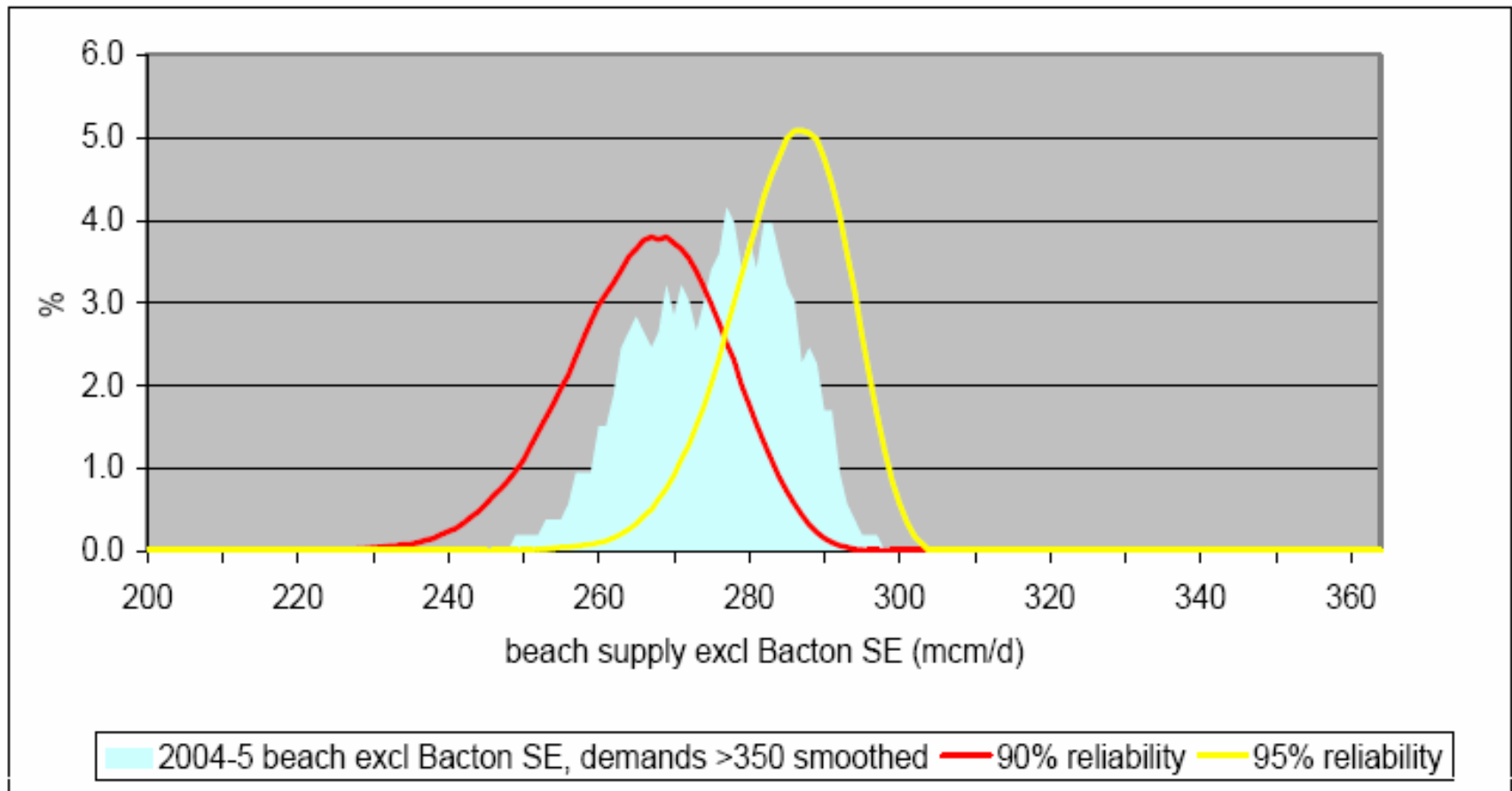
Figure 20 – Theoretical distribution v actual distribution of beach delivery in 2004/05
