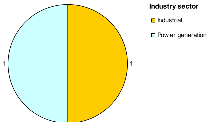
Figure 10: General industry sectors that affect 1a and 1b transitional water bodies (abstraction pressures)
