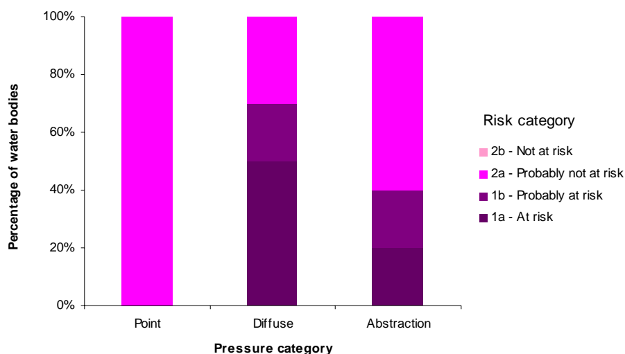
Figure 18: Pressures acting on groundwater bodies
