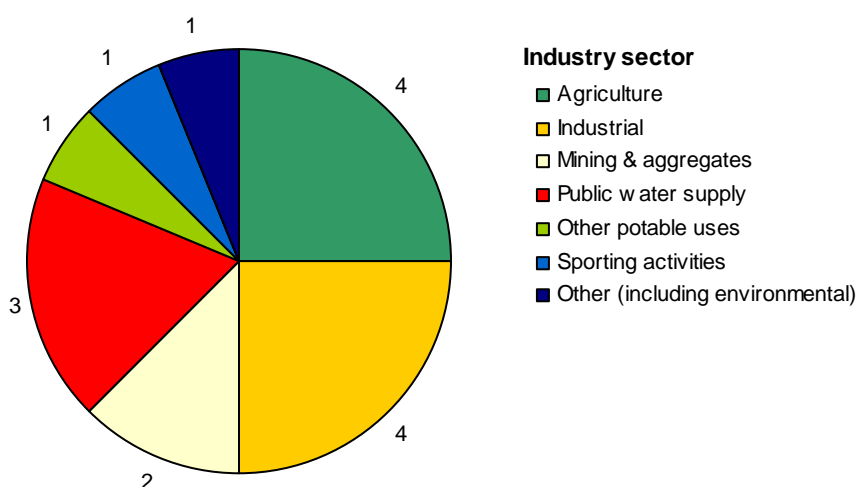
Figure 11: General industry sectors that affect 1a and 1b groundwater bodies (abstraction pressures)
