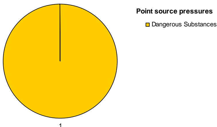
Figure 3: Point source pressures in 1a and 1b coastal water bodies
