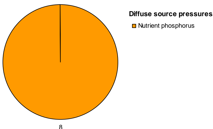
Figure 5: Diffuse source pressures in 1a and 1b lake water bodies
