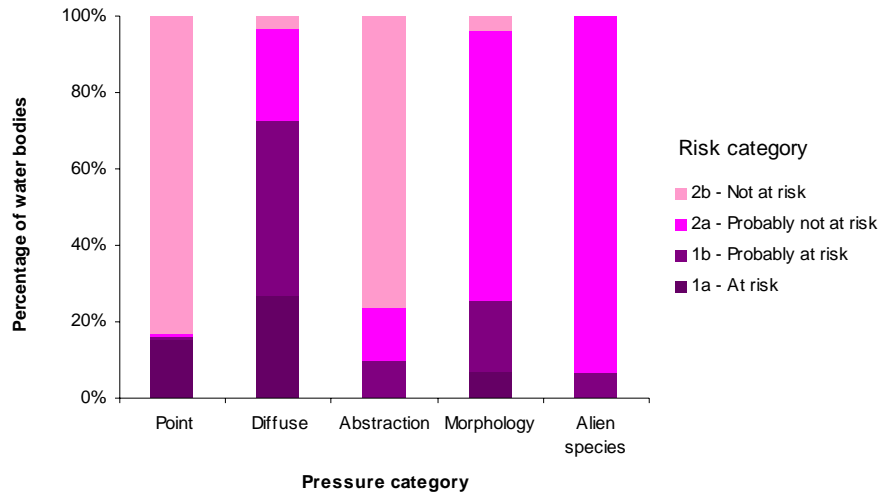
Figure 15: Pressures acting on lake water bodies
