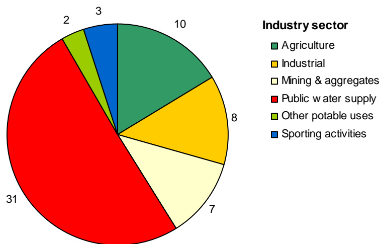
Figure 9: General industry sectors that affect 1a and 1b river water bodies (abstraction and flow-regulation pressures)
