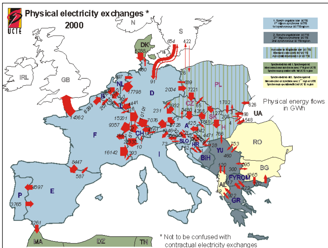
Fig. 5: Physical electricity exchanges within UCTE (UCTE 2000)
