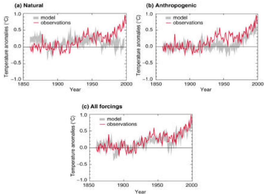
Figure A1. Comparison of outputs from climate model compared with observations of global temperature change under different forcing scenarios.
