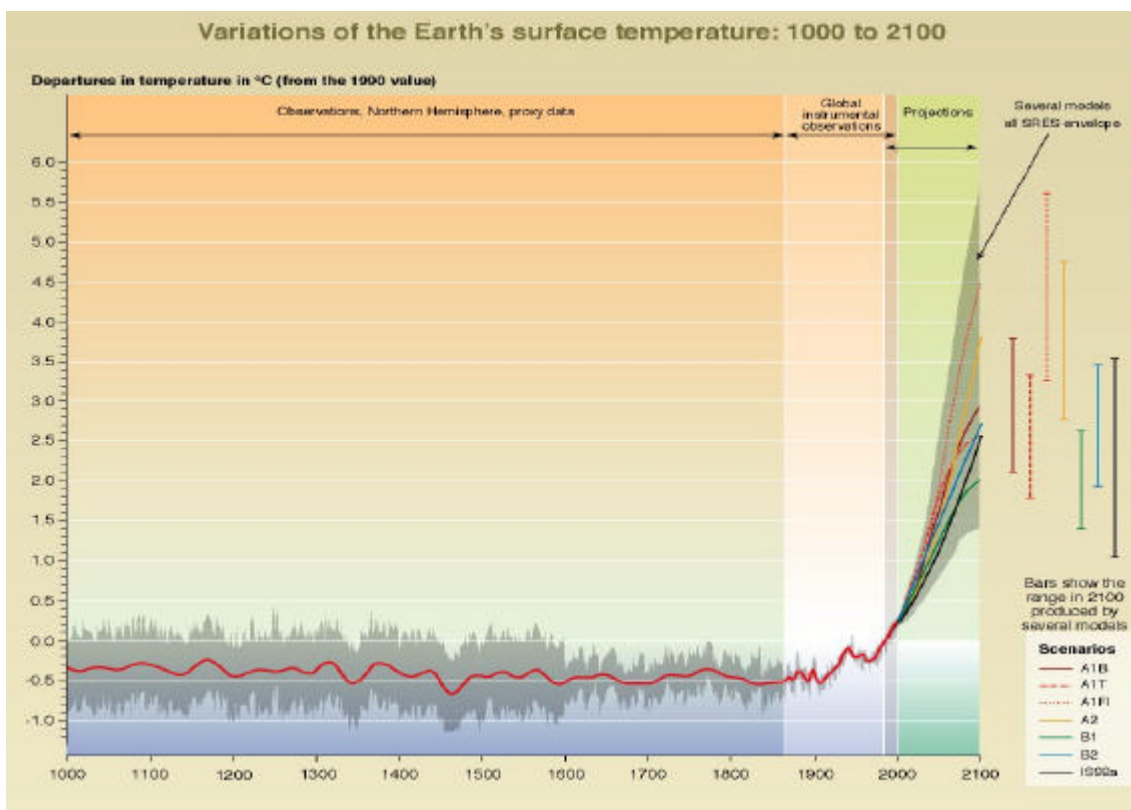
Figure A2. Projected changes in global average temperature to 2100 under different emissions scenarios (highest – A1FI, lowest – B1).
