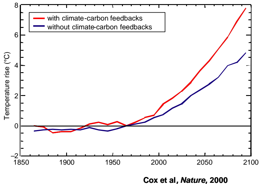
Figure A7. Increase in global temperature with and without carbon cycle feedbacks. The red line include dieback of the Amazon forest and other vegetation sources – which release carbon into the atmosphere and change from becoming a sink to a source of carbon.
