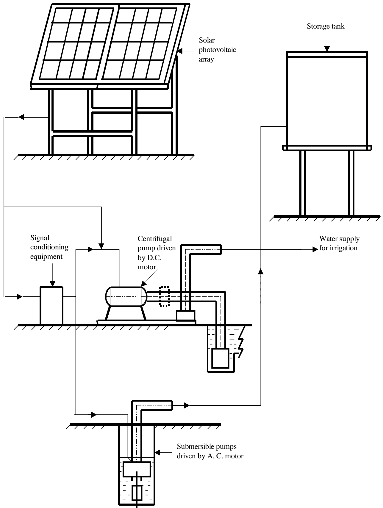
Figure 2. Schematic diagram of solar photovoltaic water pump
