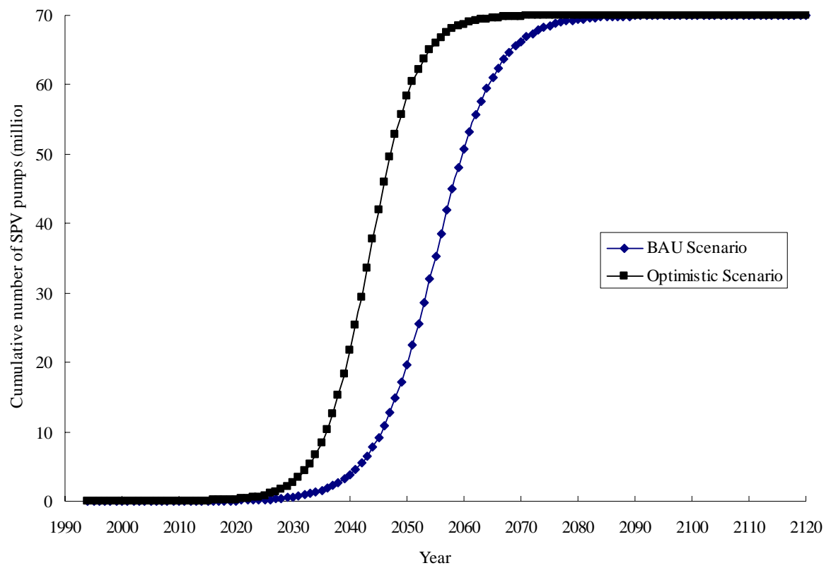
Figure 4. Time variation of cumulative number of installation of SPV pumps in India using Logistic model
