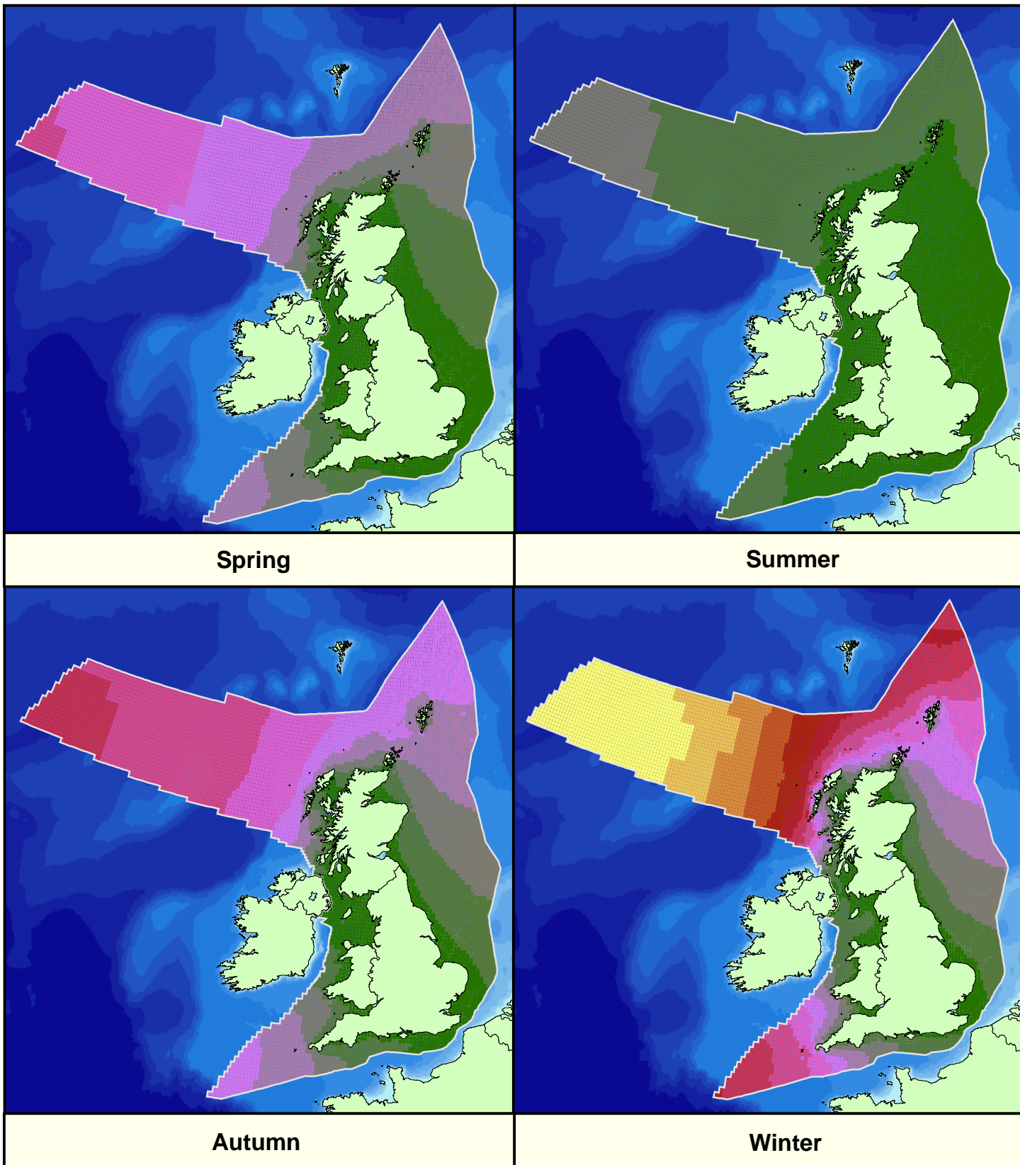
Figure 12 - Seasonal Variations in Mean Wave Power
