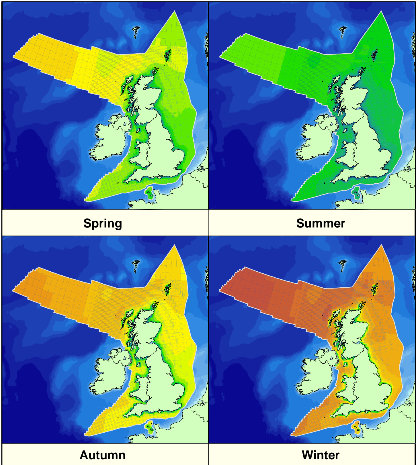
Figure 14 - Seasonal Mean Wind Speed
