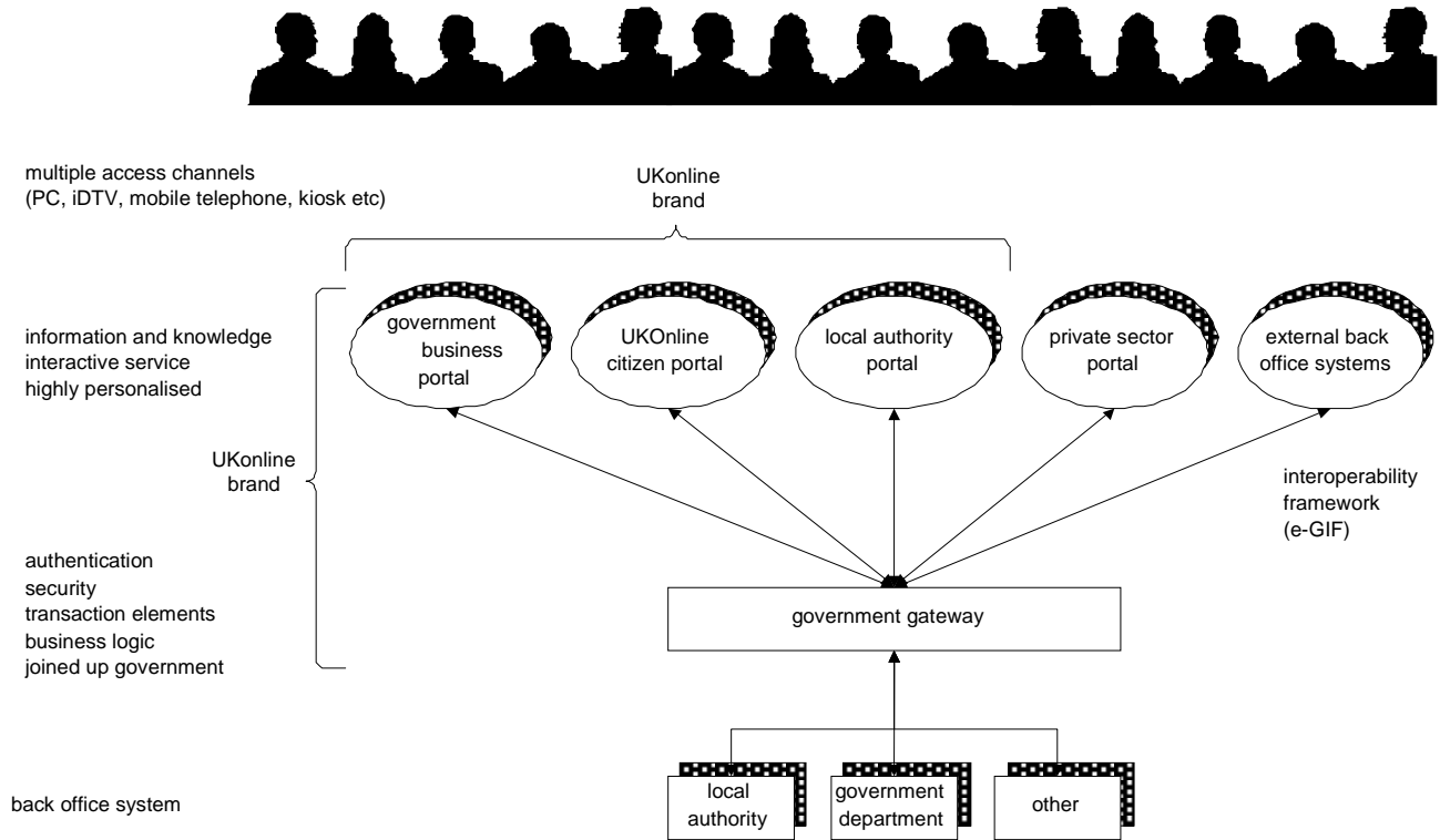
Figure 1: Portal and government gateway architecture
