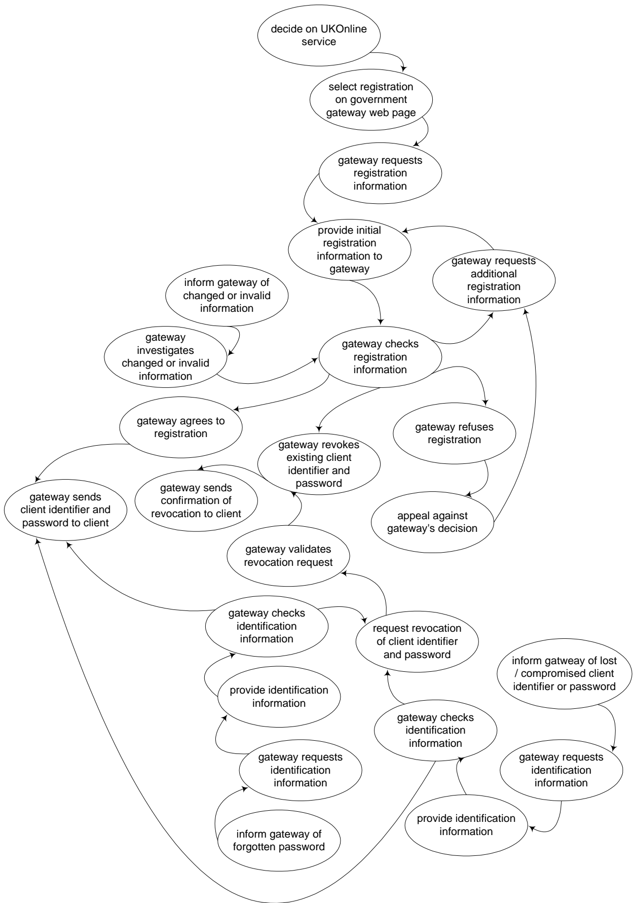
Figure 5: Scenario S1: the concept of operations for registration
