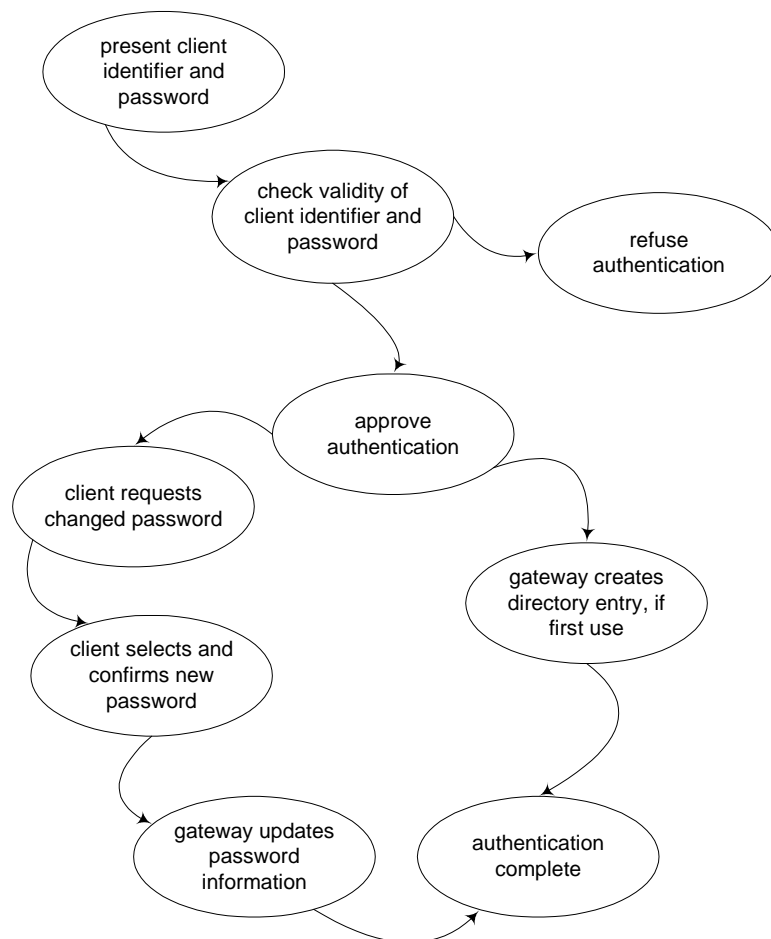
Figure 6: Scenario S1: the concept of operations for enrolment at the government gateway
