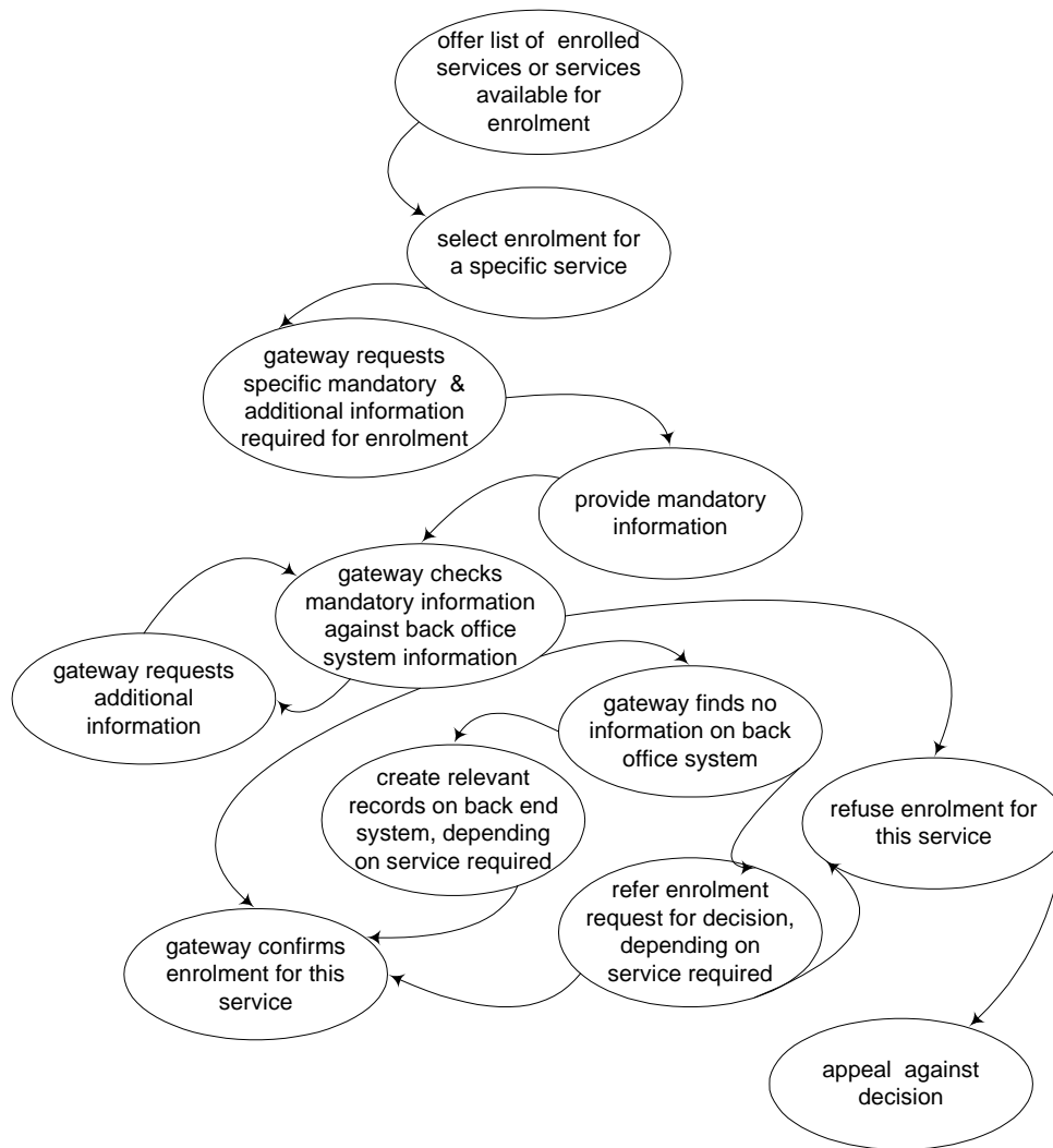
Figure 7: Scenario S1: the concept of operations for enrolment
