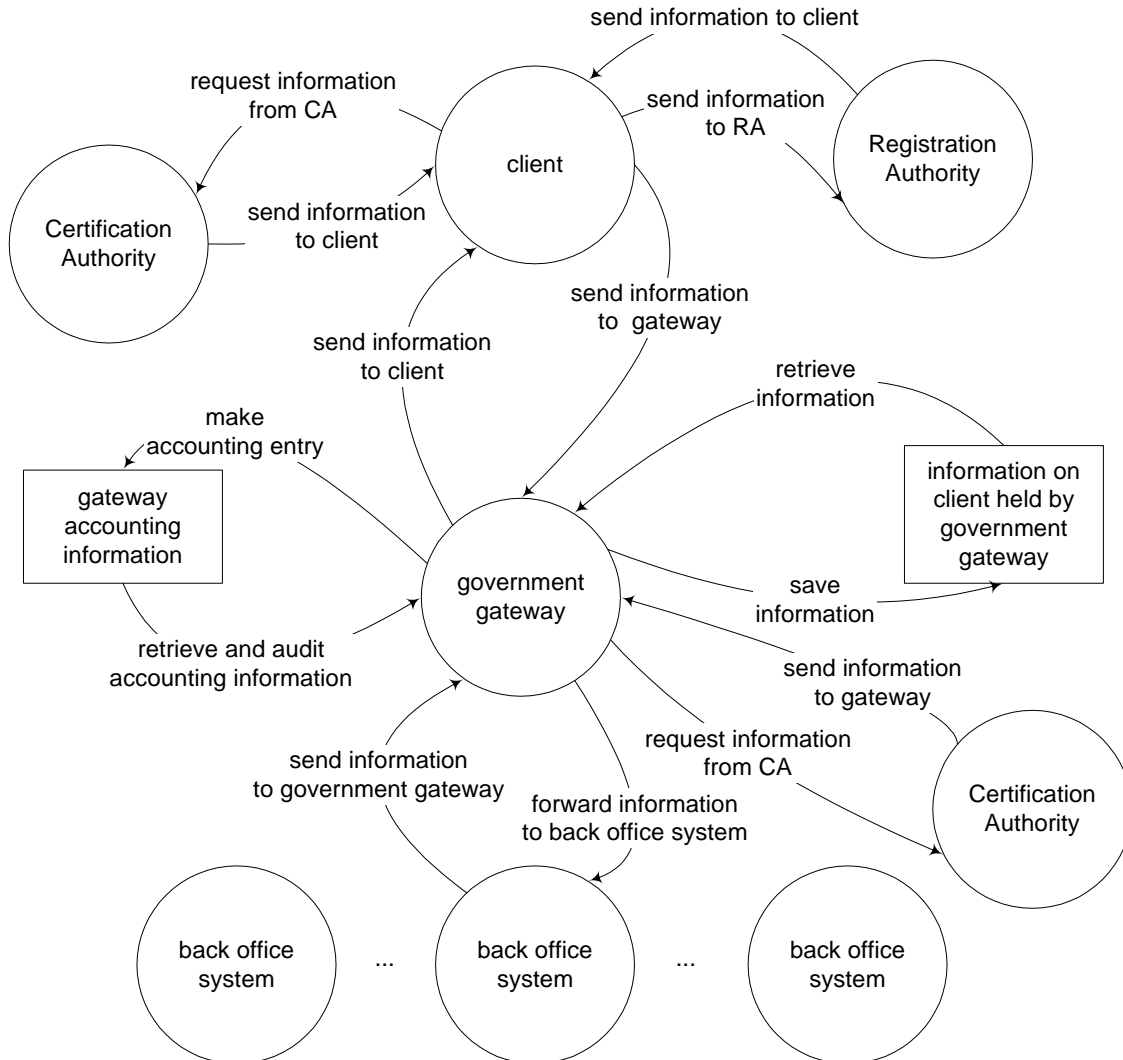
Figure 4: Overview of the supporting functions for the security architecture for the government gateway
