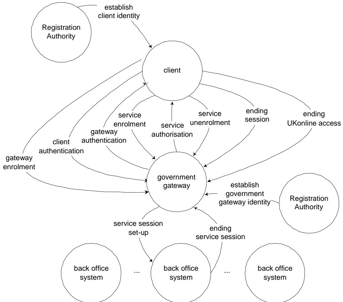
Figure 3: Overview of the security architecture for the government gateway
