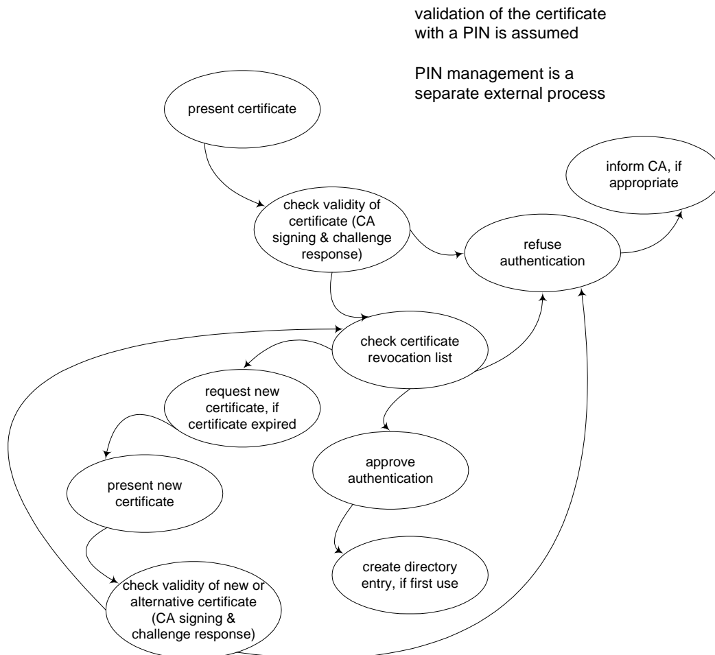
Figure 9: Scenario S2: the concept of operations for government gateway enrolment
