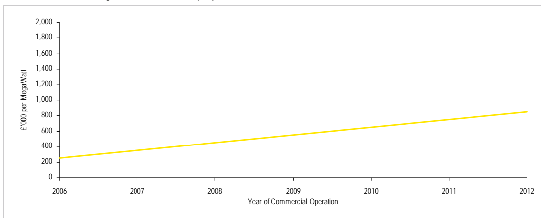
Figure 5: Foundation cost at COD – indicative trend line 2006-2012
