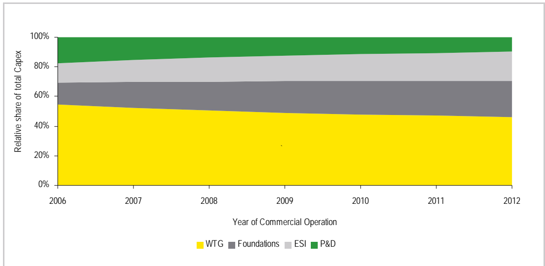
Figure 3: Material Costs as a proportion of total capital costs over time
