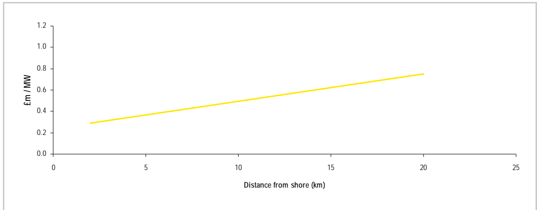
Figure 6: Electrical infrastructure cost vs. distance from shore
