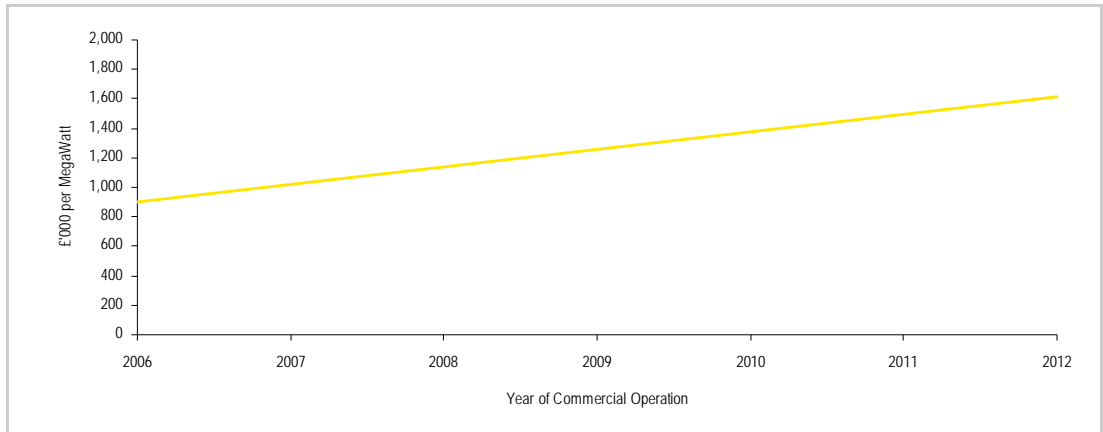
Figure 4: WTG cost at COD – indicative trend line 2006-2012
