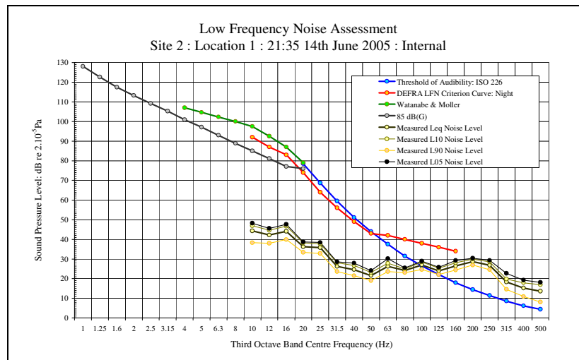
LFN Audibility Internal Before Windows Open 14/06/06 Figure 8
