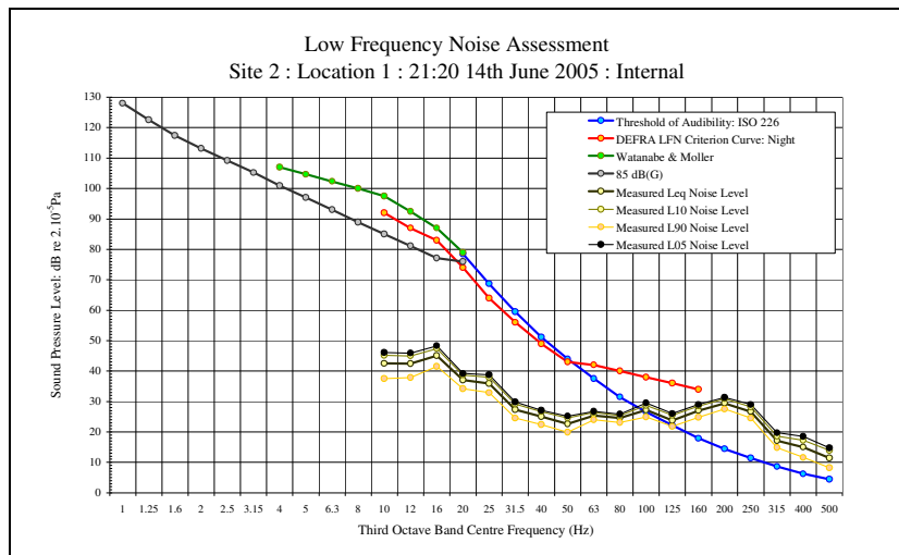
LFN Audibility Internal Before Windows Open 14/06/06 Figure 5
