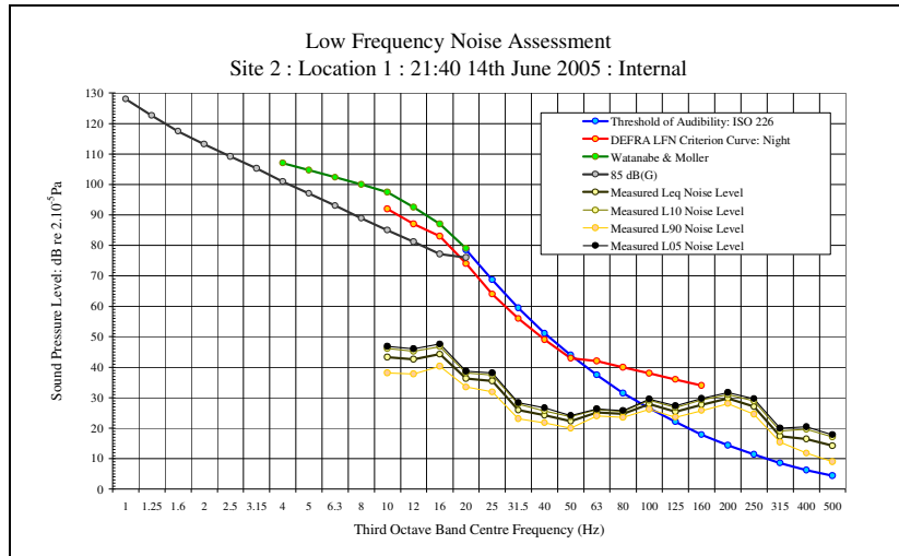
LFN Audibility Internal Before Windows Open 14/06/06 Figure 9
