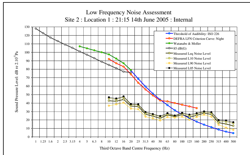
LFN Audibility Internal Before Windows Open 14/06/06 Figure 4
