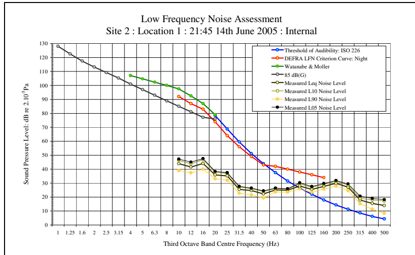
LFN Audibility Internal Before Windows Open 14/06/06 Figure 10
