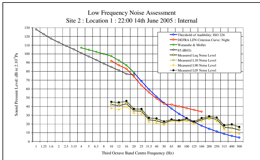
LFN Audibility Internal Before Windows Open 14/06/06 Figure 13
