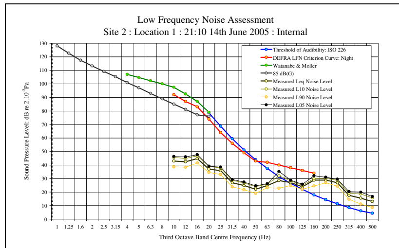
LFN Audibility Internal Before Windows Open 14/06/06 Figure 3
