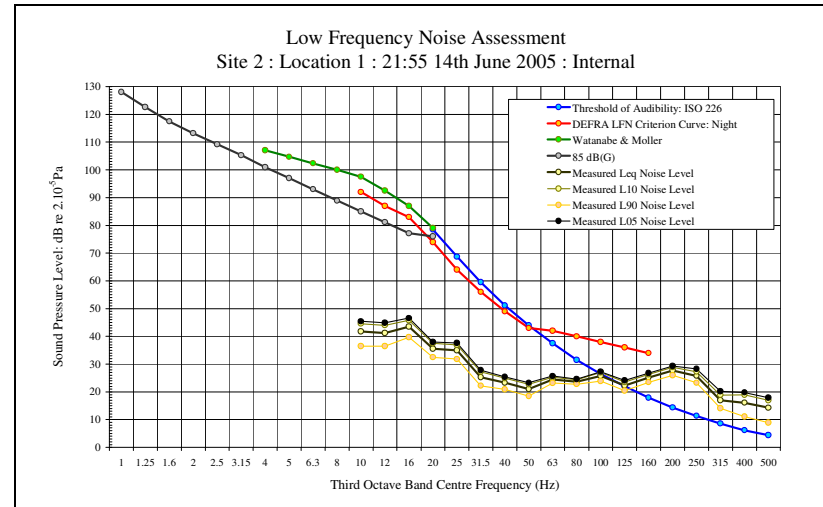
LFN Audibility Internal Before Windows Open 14/06/06 Figure 12
