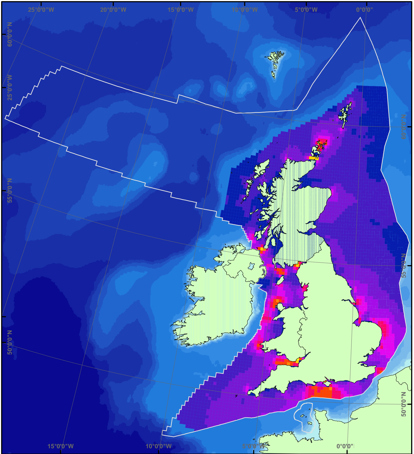
Figure B4.7 - Current Speeds extracted from the CS3 Model (depth-averaged)
