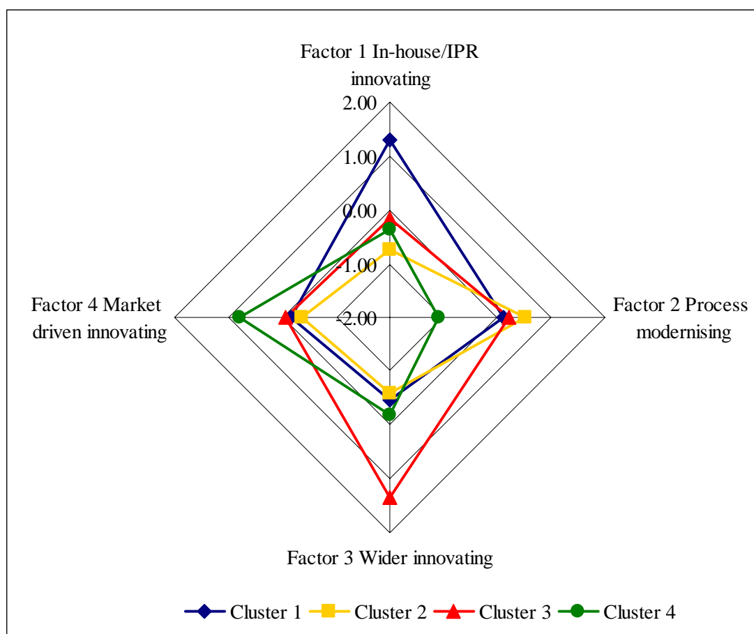
Figure 4.1 Cluster analysis
